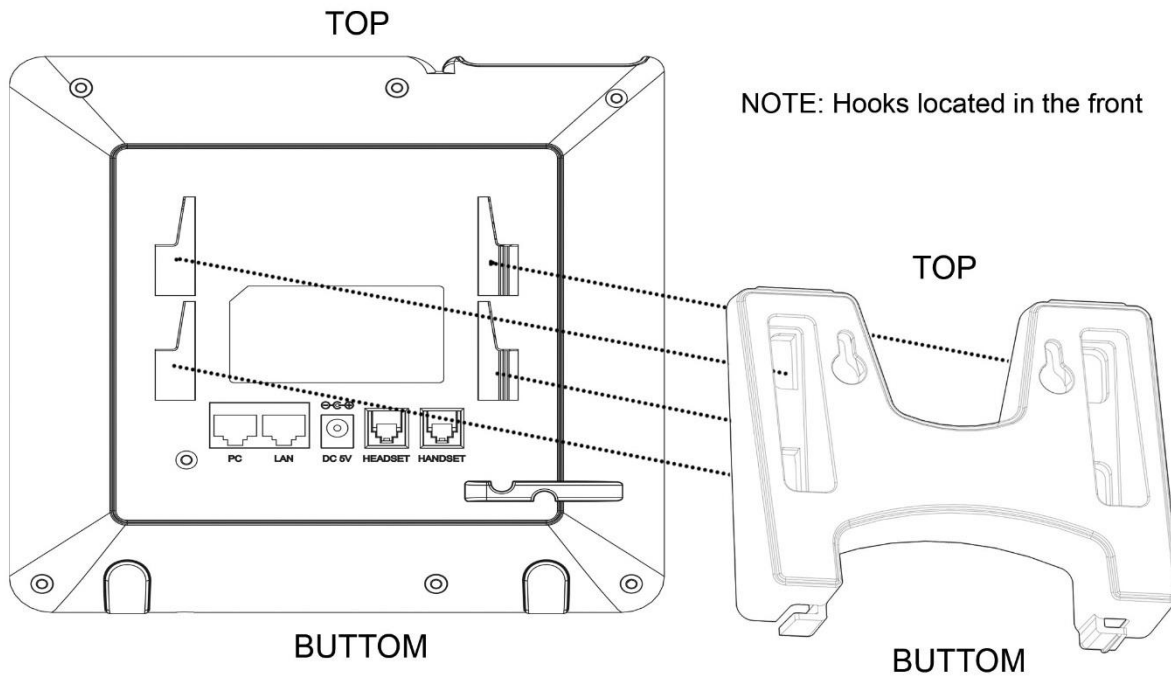
Figure 3: GXP16xx Wall Mount installation
