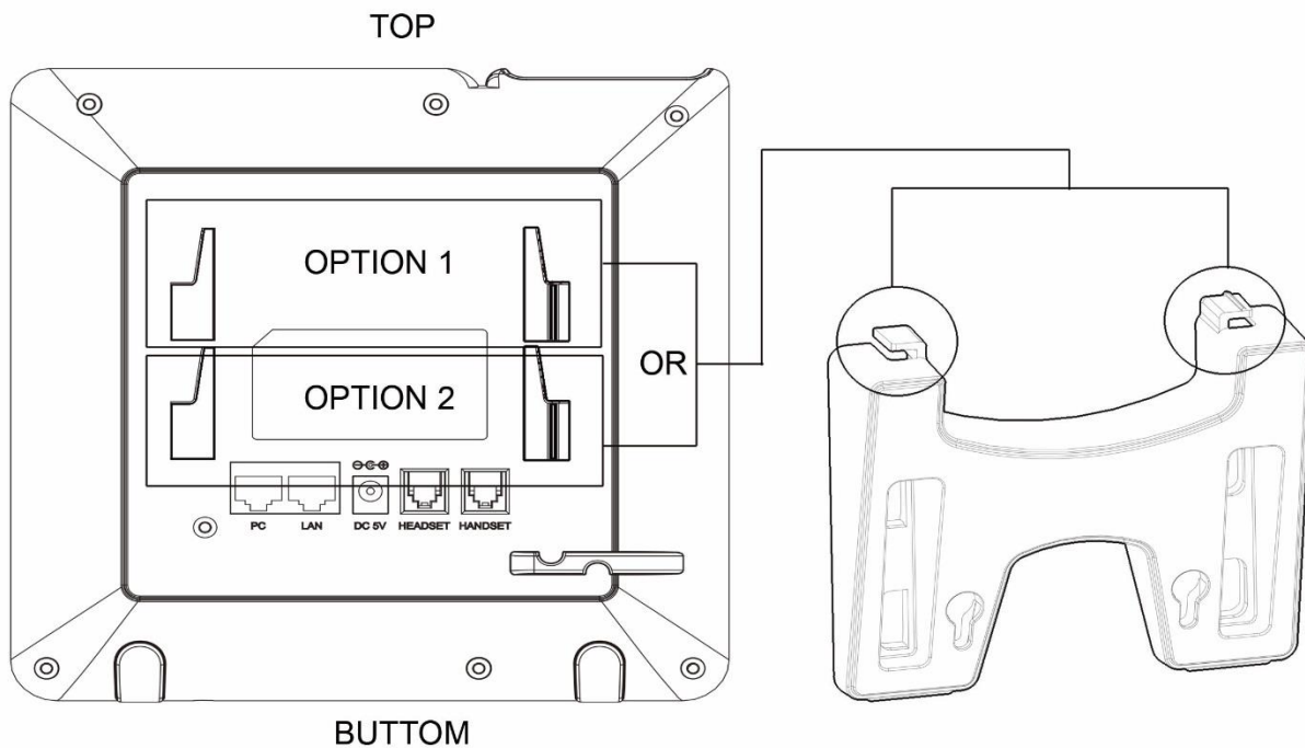
Figure 2: GXP16xx Stand Installation
